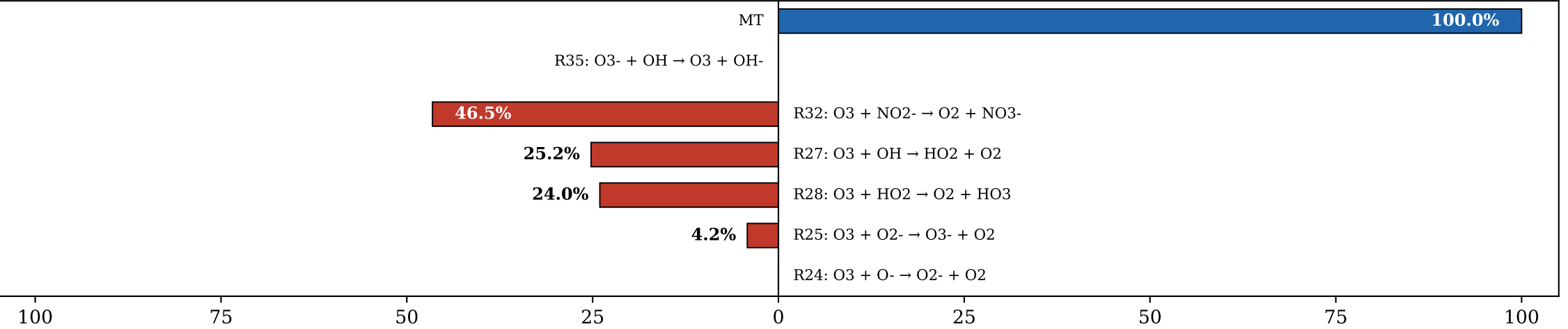
(c) NO 2 - (Σsrc = 4.25e-08 M/s)
